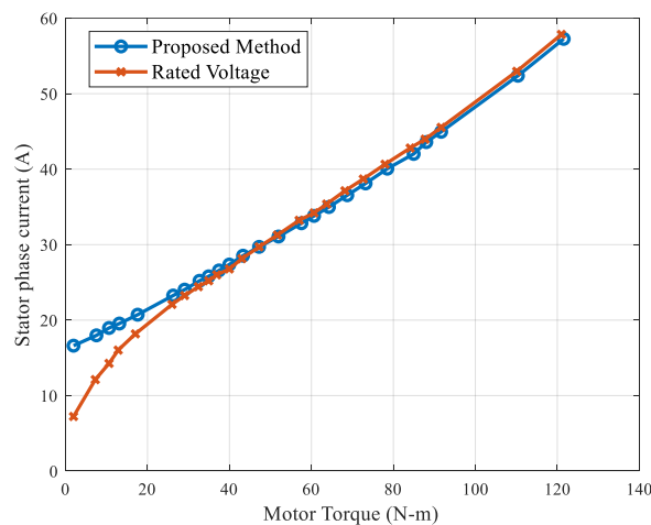
Figure 5 Outcome Simulink of stator phase verse motor torque
