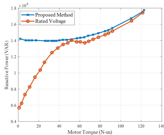
Figure 9 Outcome Simulink of Reactive power verse motor torque
